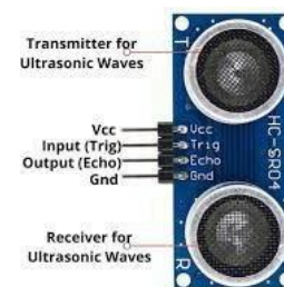
Figure.3: Ultrasonic Sensor
